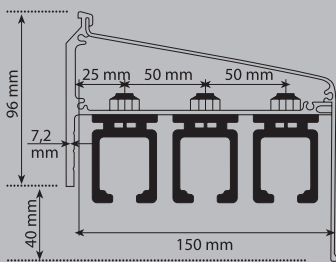
Profilkit 3-spurig
